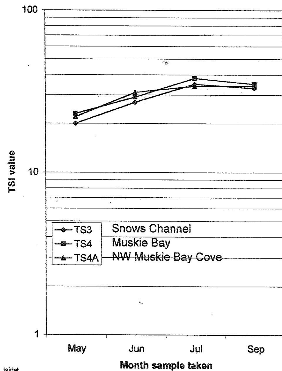
Fig. 4. Chlorophyll TSI values for sites TS3, TS4 & TS4A
