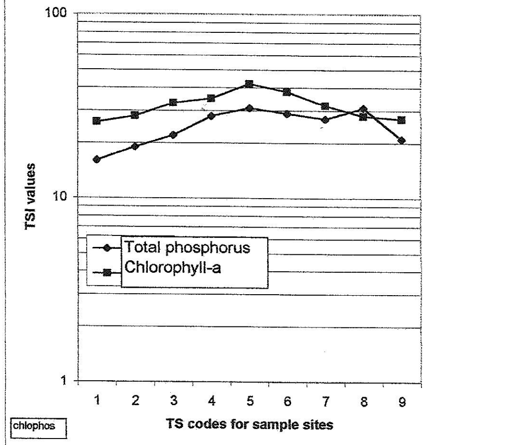
Fig. 2. Comparison of total phosphorus and chlorophyll-a TSI values for Sep, 2001 samples at nine Les Cheneaux locations.
